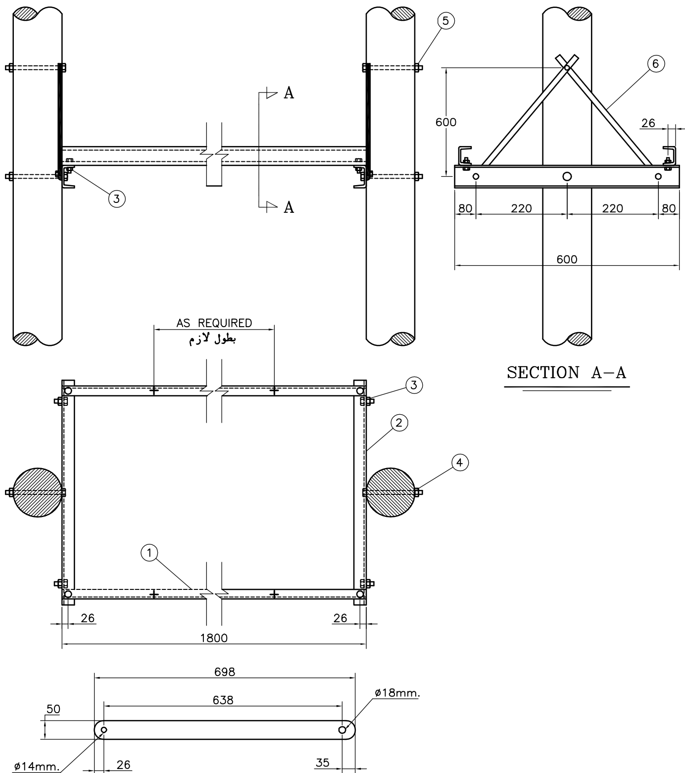
FLAT ARM BRACE
