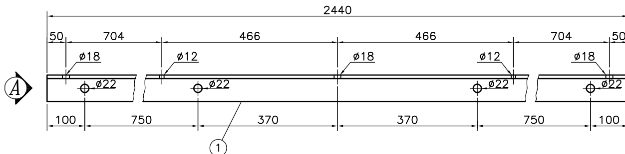
STEEL CROSS ARM
